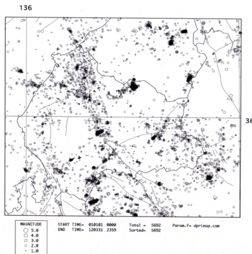
Epicenter for Reihoku Area 2001.01 - 2012.03 ( M \geq 1.0 , H \leq 30\text{km} )
