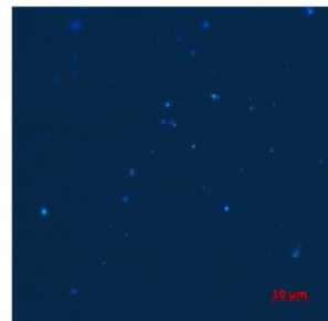
DAPI stained microbes in lake water.
