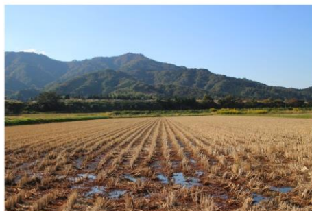
Rice paddies – a major source of methane.
