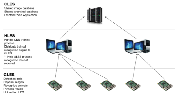
Fig: Conceptual IoT edge architecture of DHEA
