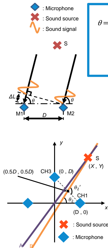
Estimation of sound source position (proposed method)
