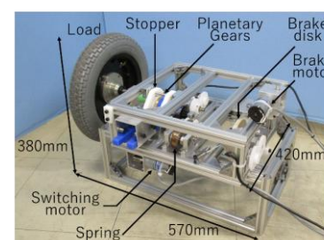
Fig.2 Experimental system
