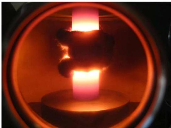
Photo. Pulse Electric Current Sintering at 1500°C
